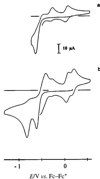
Fig. 5 Cyclic voltammetry of \text{cis-}[\text{Fe}_2(\text{cp})_2(\mu\text{-SMe})_2(\text{MeCN})_2]^{2+} \mathbf{2}^{2+} in MeCN-[NBu 4 ][PF 6 ] under CO (1 atm) showing (a) the formation of the cis dicarbonyl and (b) the formation of cis - and trans - [\text{Fe}_2(\text{cp})_2(\mu\text{-SMe})_2(\text{CO})_2] when the potential range includes both reduction steps (scan rate 0.2 \text{ V s}^{-1} ; vitreous carbon electrode).
