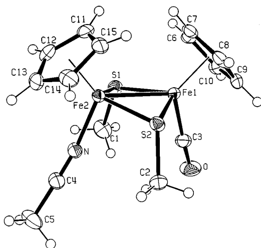
Fig. 1 A view of the dication in cis -[Fe 2 (cp) 2 (μ-SMe) 2 (CO)(MeCN)]-[BF 4 ] 2 ·CH 2 Cl 2 3 showing 50% thermal ellipsoids for non-hydrogen atoms.
