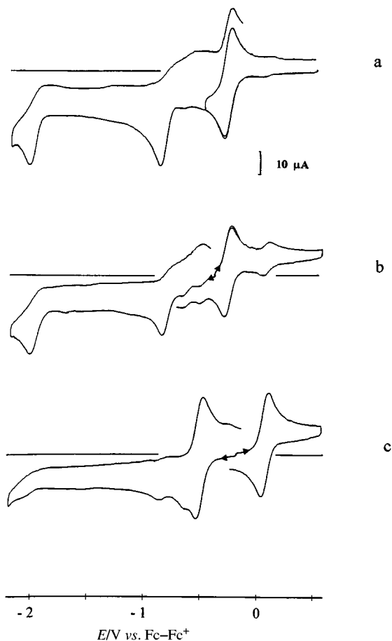
Fig. 2 Cyclic voltammetry of cis\text{-}[\text{Fe}_2(\text{cp})_2(\mu\text{-SMe})_2(\text{CO})(\text{MeCN})]^{2+} 3^{2+} (1.3 mM in \text{MeCN}\text{-}[\text{NBu}_4][\text{PF}_6] ) (a) before and (b) after controlled-potential reduction at -0.37 V (platinum cathode, inert atmosphere, n = 0.68 F per mol 3^{2+} ). The solution in (c) was obtained after treatment of that solution in (b) with CO (scan rate 0.2 V \text{s}^{-1} ; vitreous carbon electrode).
